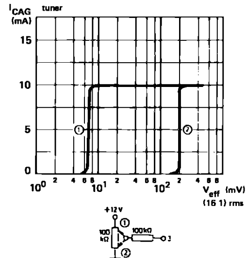
TDA2541
