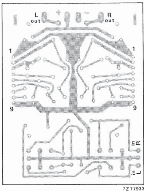
Fig.13 Track side of printed-circuit board used for the circuit of Fig.12; p.c. board dimensions 83 mm × 65 mm.
