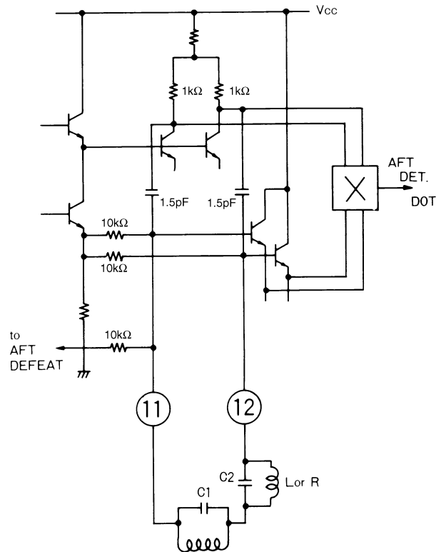
Figure 18. AFT tank
