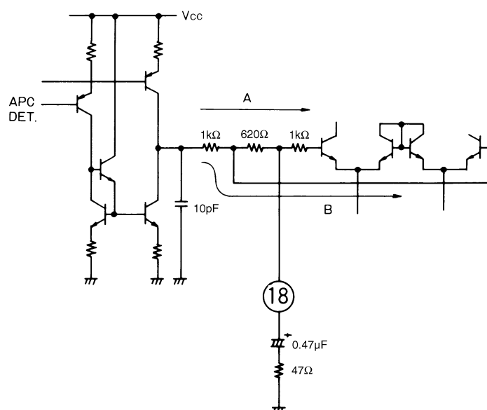
Figure 23. APC filter
