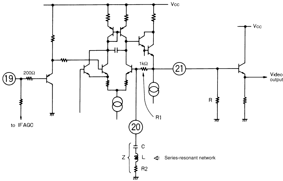
Figure 24. Equalization amplifier
