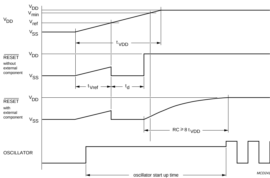
Fig.7 Reset with slow V_{DD} .
