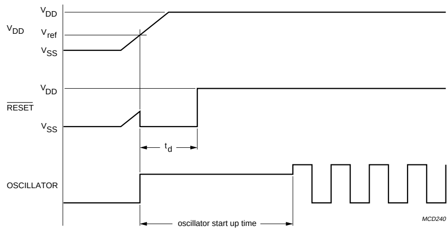
Fig.6 Reset with fast rising V_{DD} .
