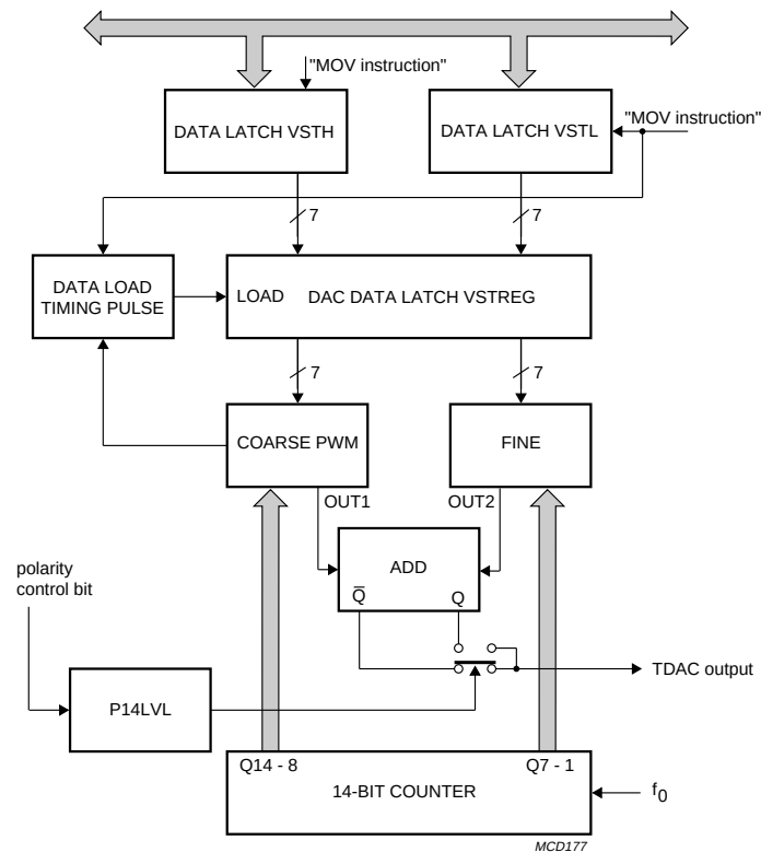
Fig.10 Block diagram of the 14-bit PWM DAC.
