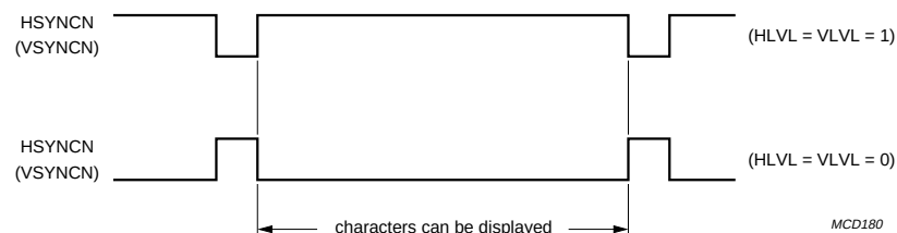
Fig.21 VSYNCN and HSYNCN active level.
