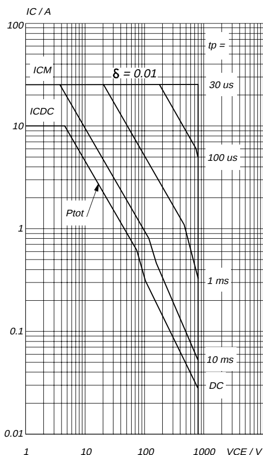
Fig.13. Forward bias safe operating area. T_{hs} = 25\text{ }^{\circ}\text{C} I_{CDC} & I_{CM} = f(V_{CE}) ; I_{CM} single pulse; parameter t_p Second-breakdown limits independent of temperature. Mounted with heatsink compound.
