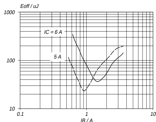
Fig.9. Typical turn-off losses. T_J = 85^\circ\text{C} E_{off} = f(I_B) ; parameter I_C ; parameter frequency
