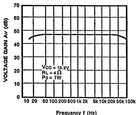
Fig. 6 - VOLTAGE GAIN vs. FREQUENCY
