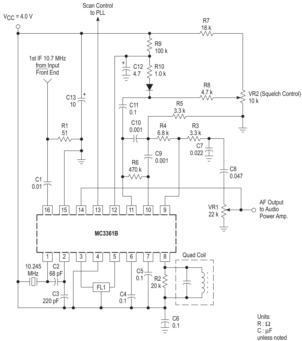
Figure 10. Simplified Application
