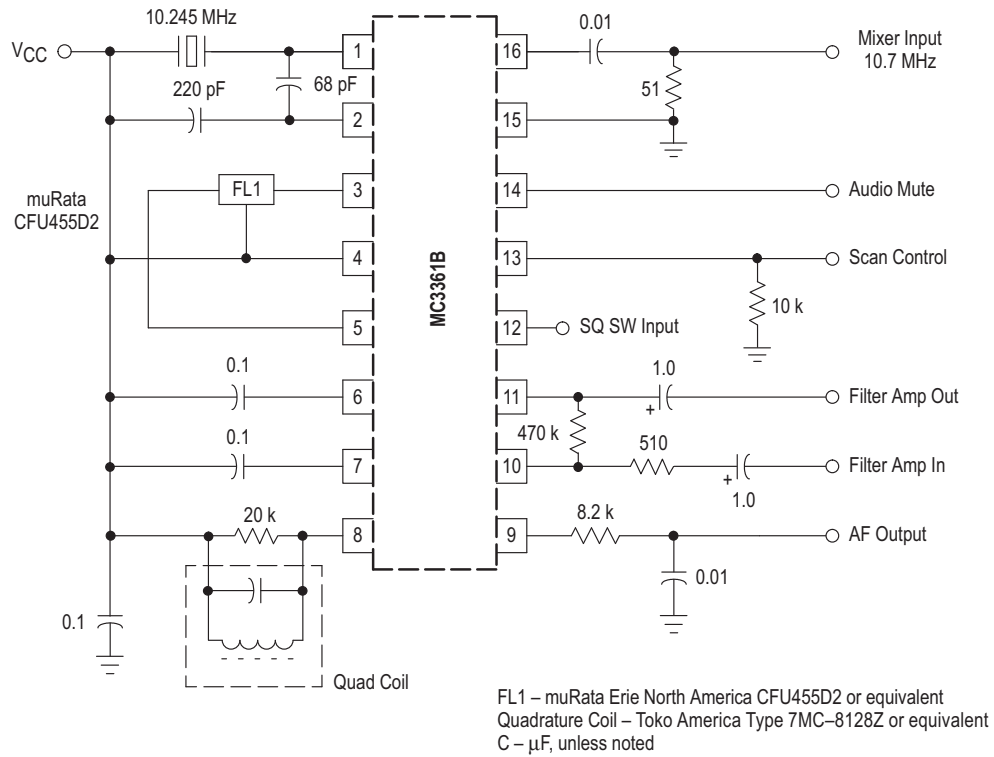
Figure 1. Test Circuit
