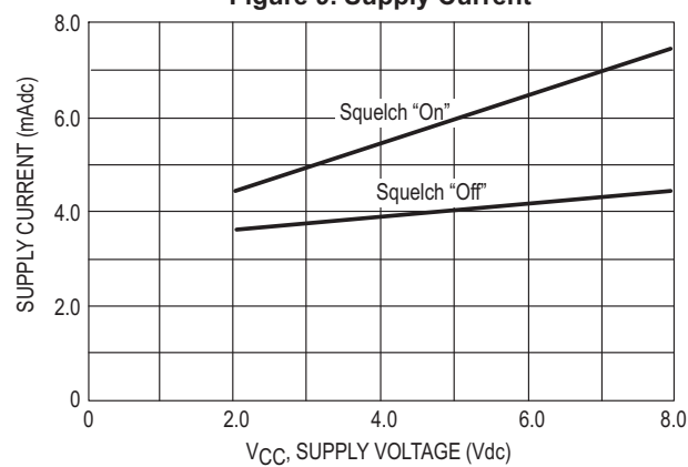
Figure 9. Supply Current
