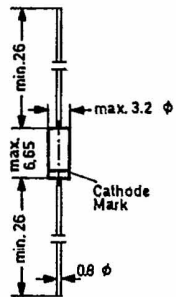
Diode Plastic Package P1 Weight approx. 0.4 g
