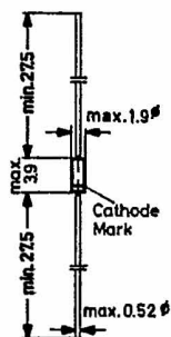
DO-35 Glass Case Weight approx. 0.13 g
