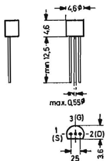
TO-92 Plastic Package (10D3) Pins in-Line "A" Weight approx. 0.18 g
