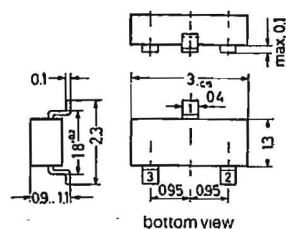
TO-236 Plastic Package (23A3) Weight approx. 0.01 g
