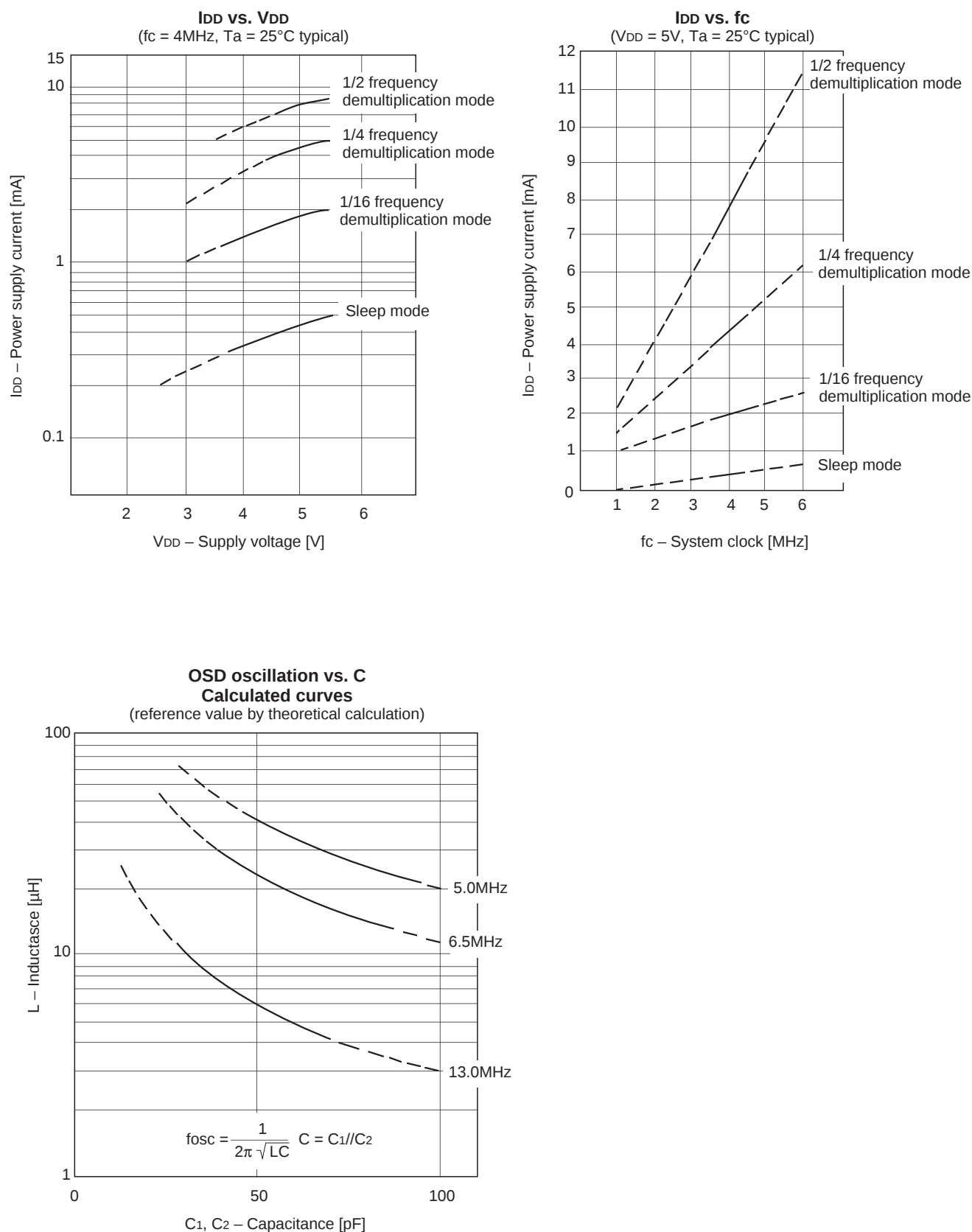
Fig. 14. Characteristics curves
