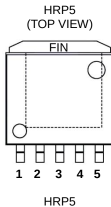
Figure 6. Pin Descriptions (Without SW) (HRP5)
