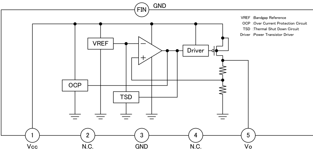
Figure 10. Block diagram BDxxC0AHFP-C (Output Voltage Fixation Type, Without SW)
