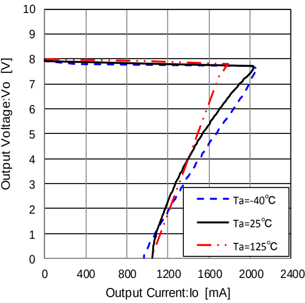
Figure 50. Load Regulation
