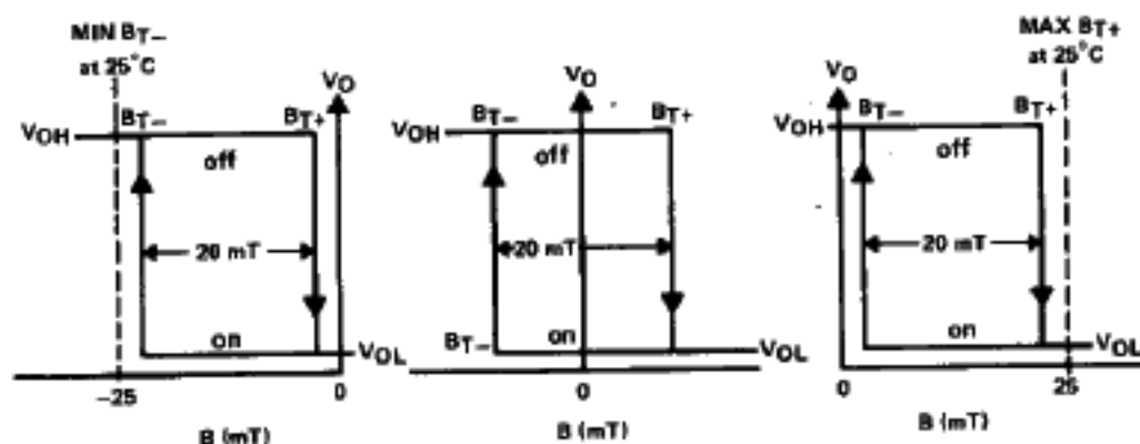
FIGURE 1. DEFINITION OF MAGNETIC FLUX POLARITY
