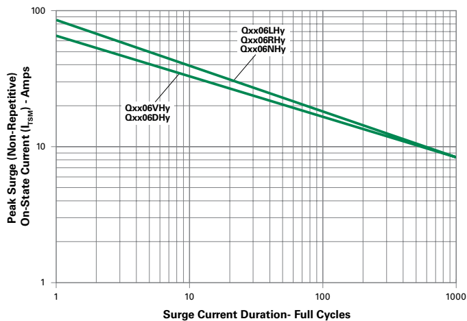
Figure 13: Surge Peak On-State Current vs. Number of Cycles (Alternistor Triac)
