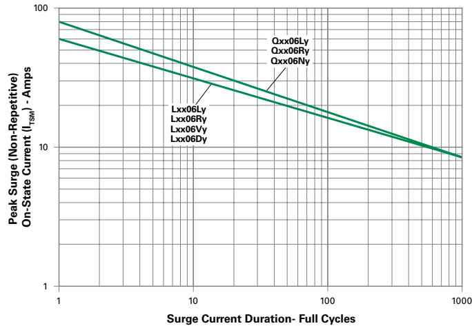
Figure 12: Surge Peak On-State Current vs. Number of Cycles (Sensitive / Standard Triac)
