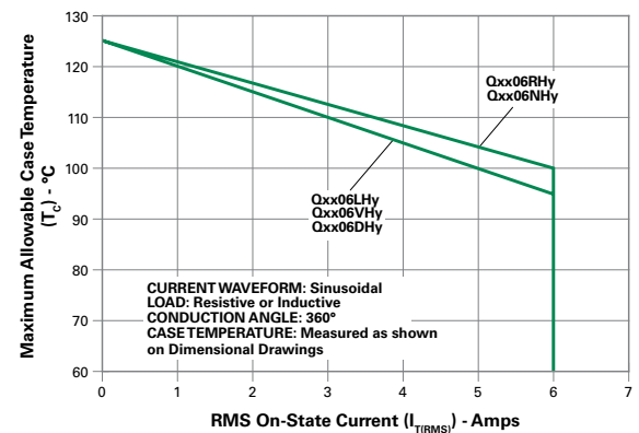
Figure 8: Maximum Allowable Case Temperature vs. On-State Current (Alternistor Triac)
