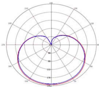
Photometric Diagram
