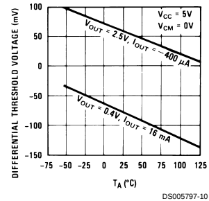
Temperature Sensitivity
