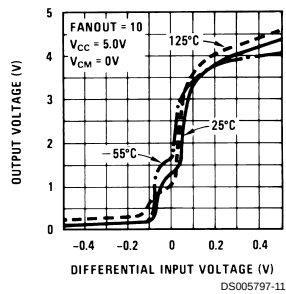
Transfer Function
