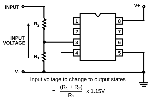
FIGURE 24. RANGE OF INPUT VOLTAGE GREATER THAN +1.15 VOLTS
