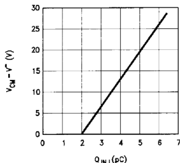
FIGURE 13. Q_{INJ} vs V_{CM} - V^-
