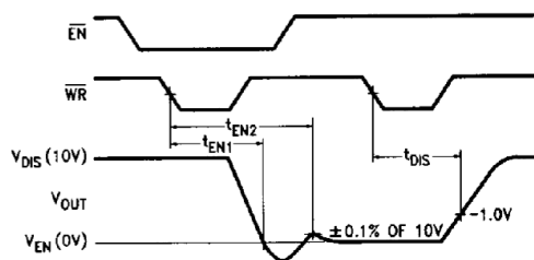
FIGURE 3. Bi-State Output Enable and Disable Time Test
