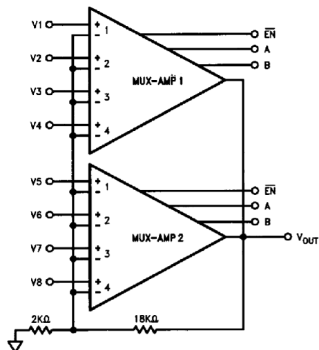
Eight Channel Multiplexer and Amplifier with a Gain of 10
