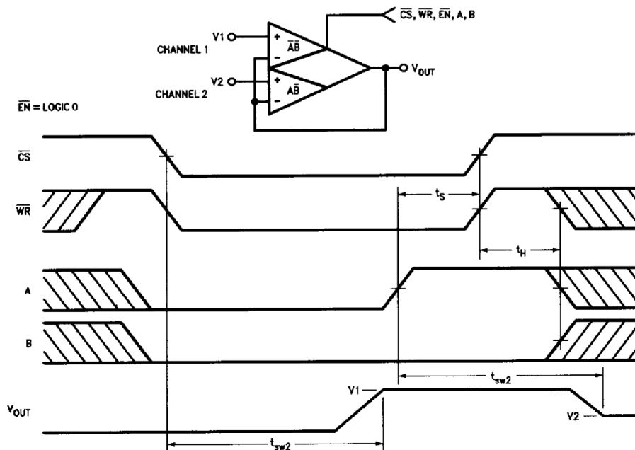
FIGURE 5. Channel Switching Timing Diagram
