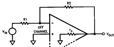
FIGURE 11. Inverting Gain Channel Feedthrough
