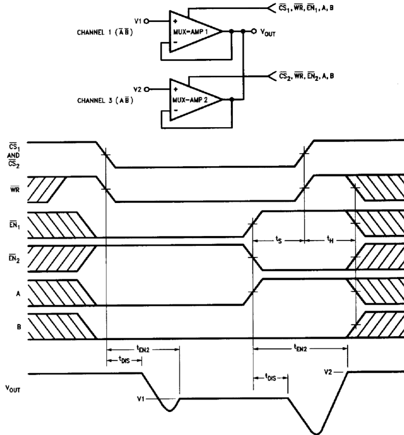
FIGURE 8. Timing Diagram for Switching Bi-State Outputs
