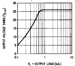
Output Voltage Swing vs Output Load Resistance
