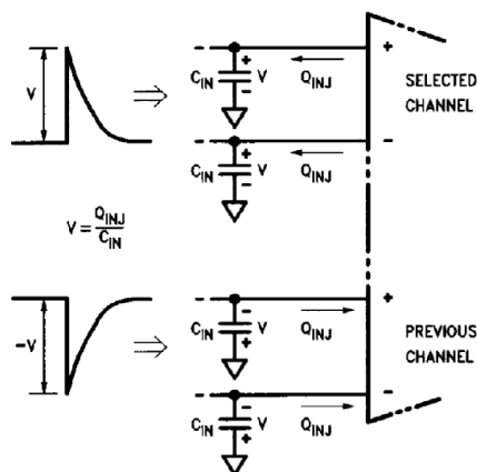
FIGURE 12. Error Voltage From Input Charge Injection
