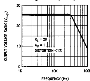
Undistorted Output Voltage Swing vs Frequency
