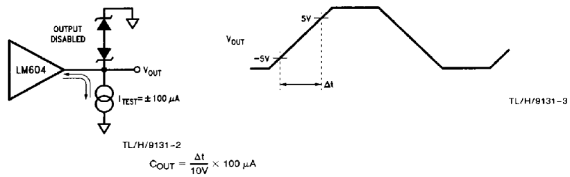
FIGURE 1. Output Capacitance Test
