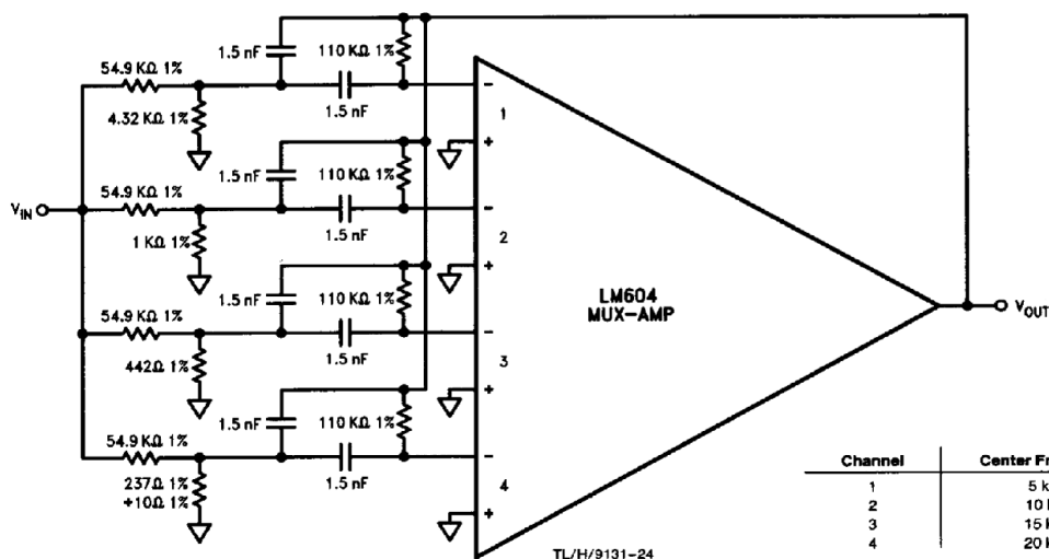
Programmable Bandpass Filter: Each channel has a 2 kHz bandwidth and a gain of 1 at the center frequency
