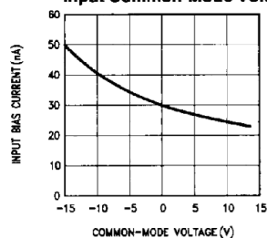
Input Bias Current vs Input Common-Mode Voltage
