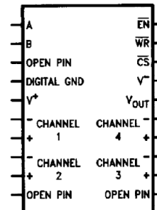
20 Pin Small Outline Package
