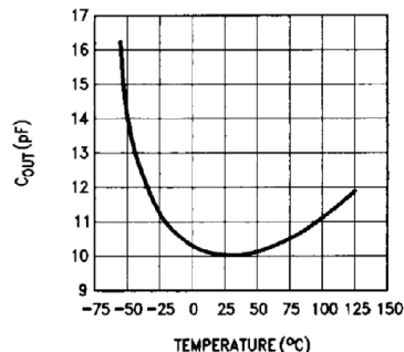
FIGURE 7. I_{LEAKAGE} and C_{OUT} vs Temperature
