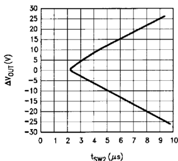
FIGURE 6. t_{SW2} vs \Delta V_{OUT}
