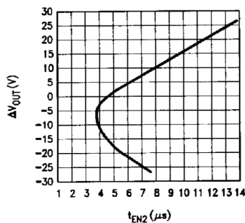
FIGURE 9. t_{EN2} vs \Delta V_{OUT}
