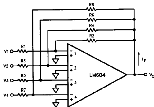
FIGURE 11. Inverting Gain Channel Feedthrough
