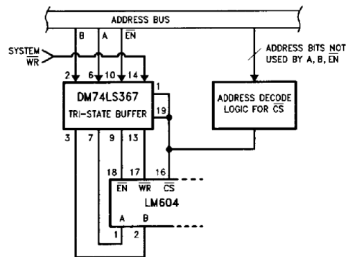
FIGURE 14. Isolating Mux-Amp from Address Bus by Using a Tri-State Buffer
