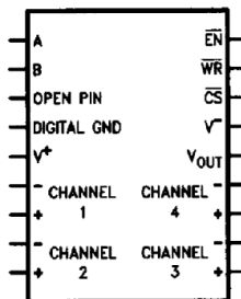
18 Pin Dual-In-Line Package
