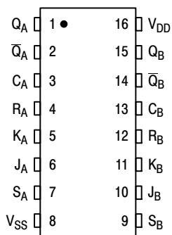
PIN ASSIGNMENT
