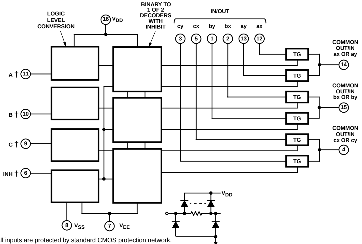
CD4053B
