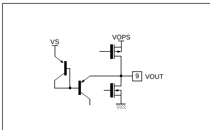
Figure 19: Vertical Output
