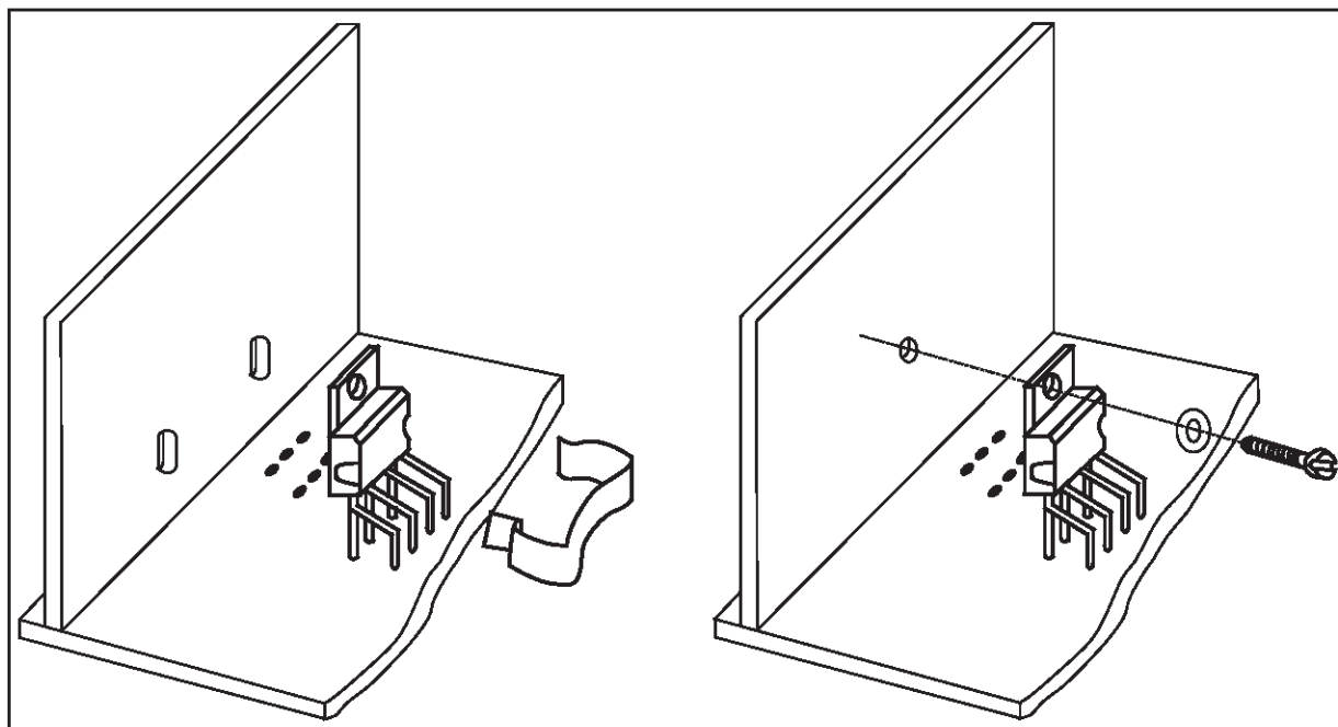
Figure 4 : Mounting Examples
