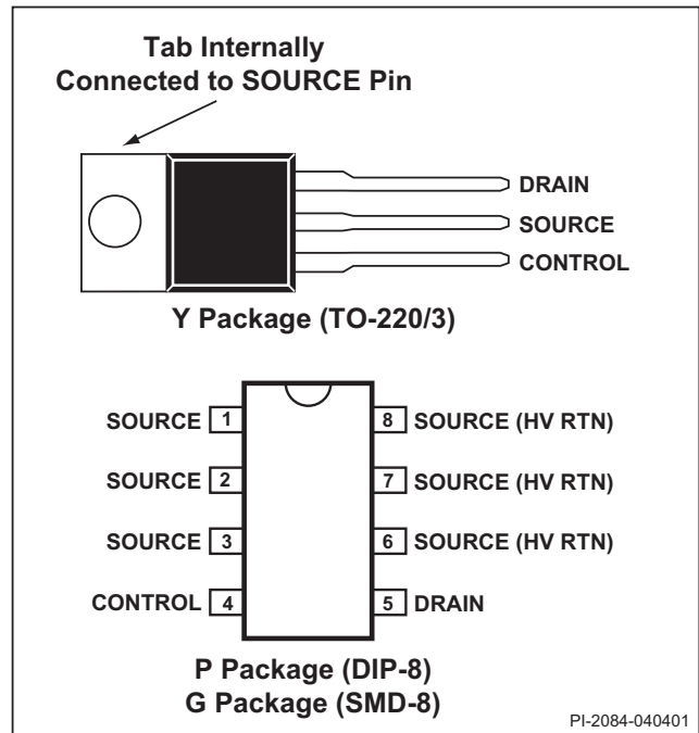
Figure 3. Pin Configuration.
