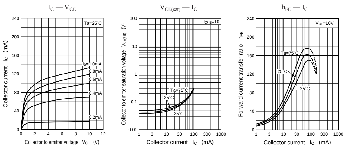
Characteristics charts of UN421L
