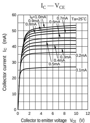
Characteristics charts of UN421E
