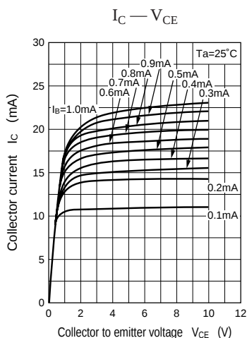
Characteristics charts of UN421D
