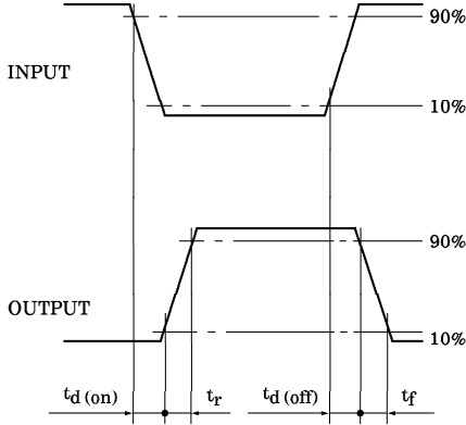
WAVEFORMS
