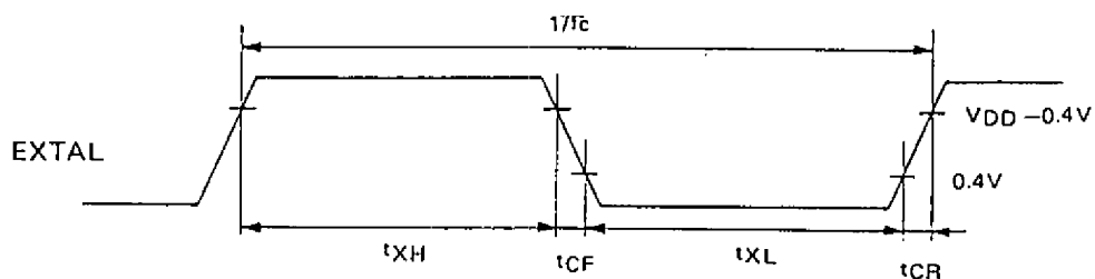
Fig. 1 Clock timing
