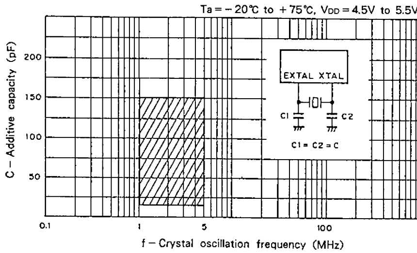
Fig. 10 Crystal oscillation circuit additive capacity calculation chart
