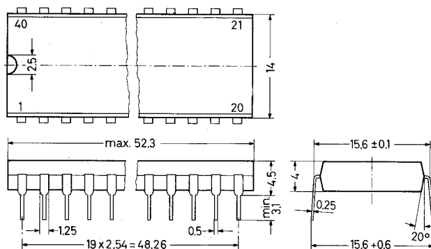
Fig. 10: VCU 2133 in 40-pin DIP Plastic Package, 20 B 40 according to DIN 41 870
