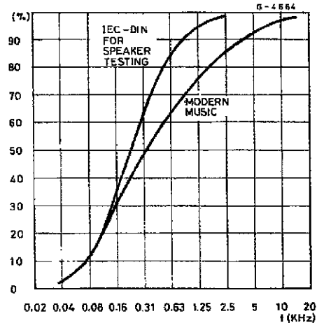
Figure 19 : Power Distribution versus Frequency
