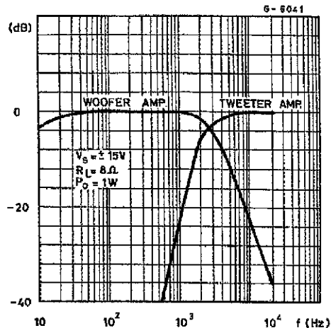
Figure 18 : Frequency Response
