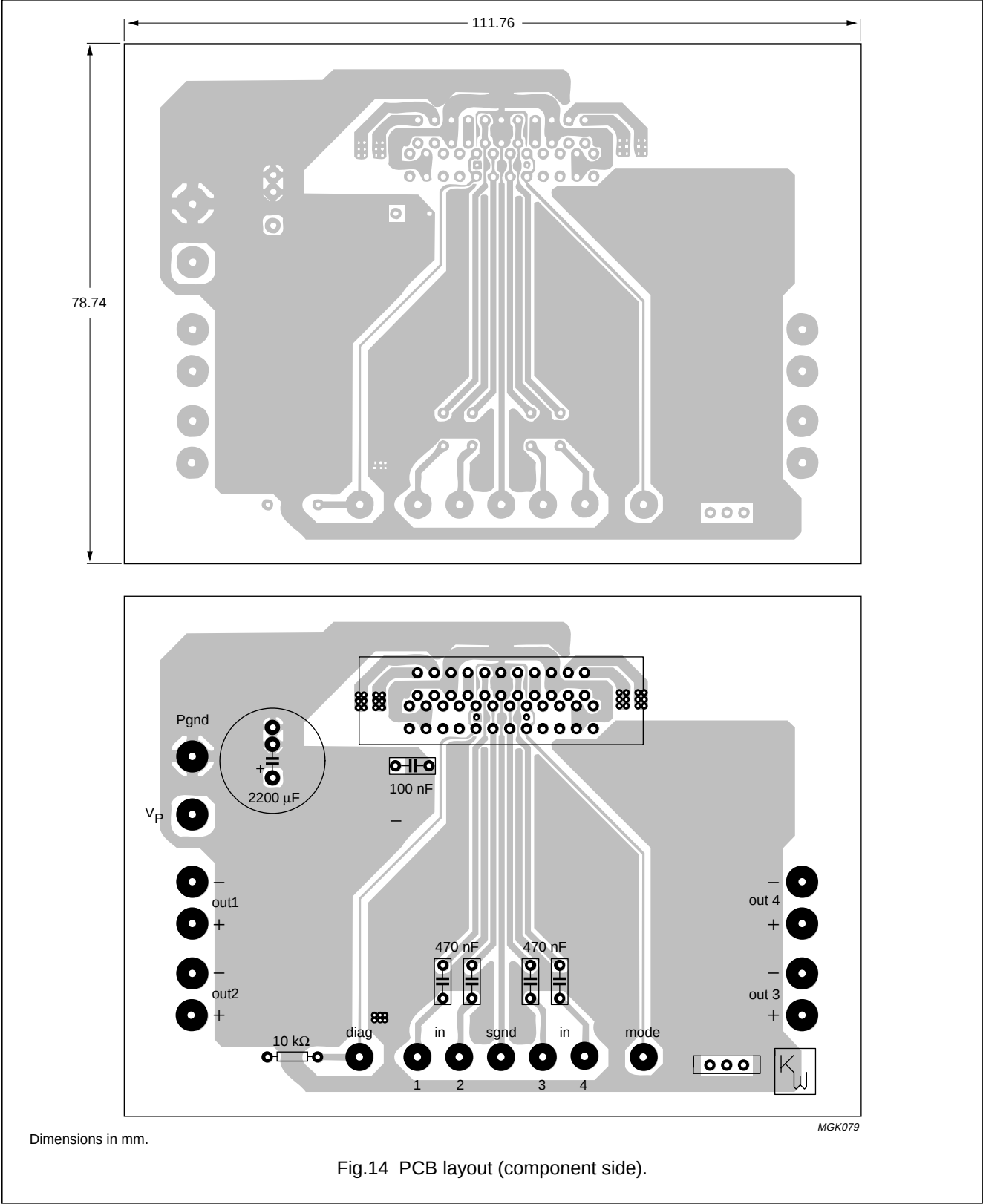
PCB layout
