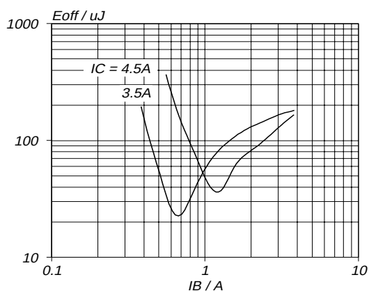
Fig.11. Typical turn-off losses. T_j = 85^\circ\text{C} E_{\text{off}} = f(I_B) ; parameter I_C
