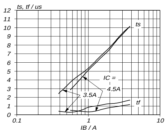
Fig.12. Typical collector storage and fall time. t_s = f(I_B) ; t_f = f(I_B) ; parameter I_C ; T_j = 85^\circ\text{C}
