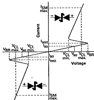
Voltage/current characteristic.
