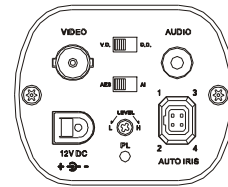
Rear Panel
