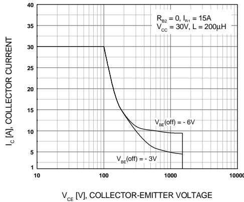
Figure 10. Reverse Bias Safe Operating Area
